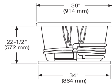
PLUMBING ROUGH-IN
