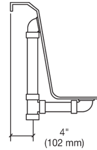
PLUMBING ROUGH-IN
