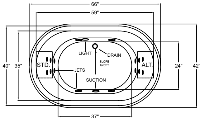
Pump locations shown for clarity. STD - Standard Location ALT - Optional Alternate Location
