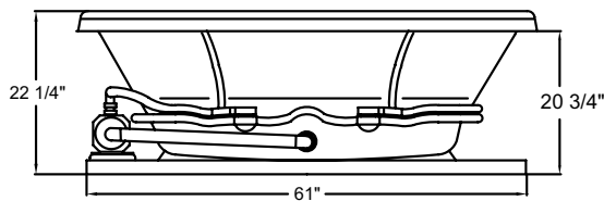
Pump locations shown for clarity. STD - Standard Location ALT - Optional Alternate Location
