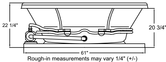
Pump locations shown for clarity. STD - Standard Location ALT - Optional Alternate Location
