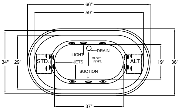
Pump locations shown for clarity. STD - Standard Location ALT - Optional Alternate Location
