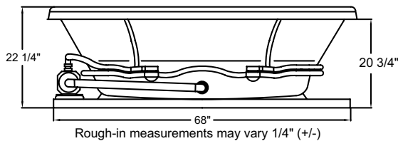
Pump locations shown for clarity. STD - Standard Location ALT - Optional Alternate Location
